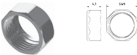
0-MU Mutter Standard screw nut (default)
