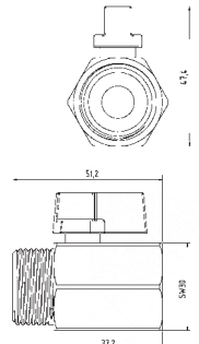
KH-34 Mini-Kugelhahn G3/4" Messing Verchromt mini ball valve thread 3/4"
