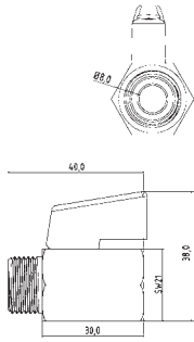
KH-38 Mini-Kugelhahn G3/8" Messing Verchromt mini ball valve thread 3/8" brass chrome-plated
