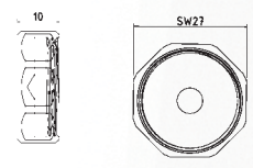
2-RSV Rückschlagventil (Drop-Stop) Check valve (Drop-Stop)
