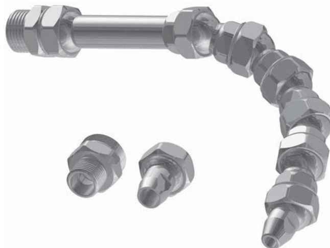
2-GS Grundset Typ2 1/2" System L = 240 mm basic set Type2 1/2" system l = 240 mm 5 x 2-GE, 1 x 2-GE-3, 1 x 2-AD-38, 1 x 2-AD-12, 1 x 2-DU-65 1 x 2-DU-10, 1 x SW-19, 1 x SW-27 5 x 2-GE, 1 x 2-GE-3, 1 x 2-AD-38, 1 x 2-AD-12, 1 x 2-DU-65 1 x 2-DU-10, 1 x SW-19, 1 x SW-27
