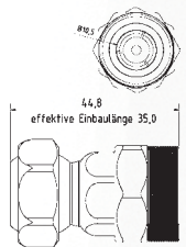
2-RSV Rückschlagventil (Drop-Stop) Check valve (Drop-Stop)
